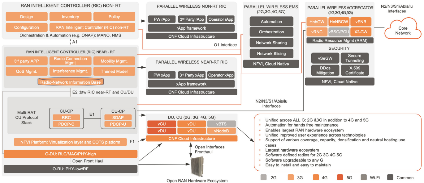
Figure 2: Complete Open RAN Solution Suite
